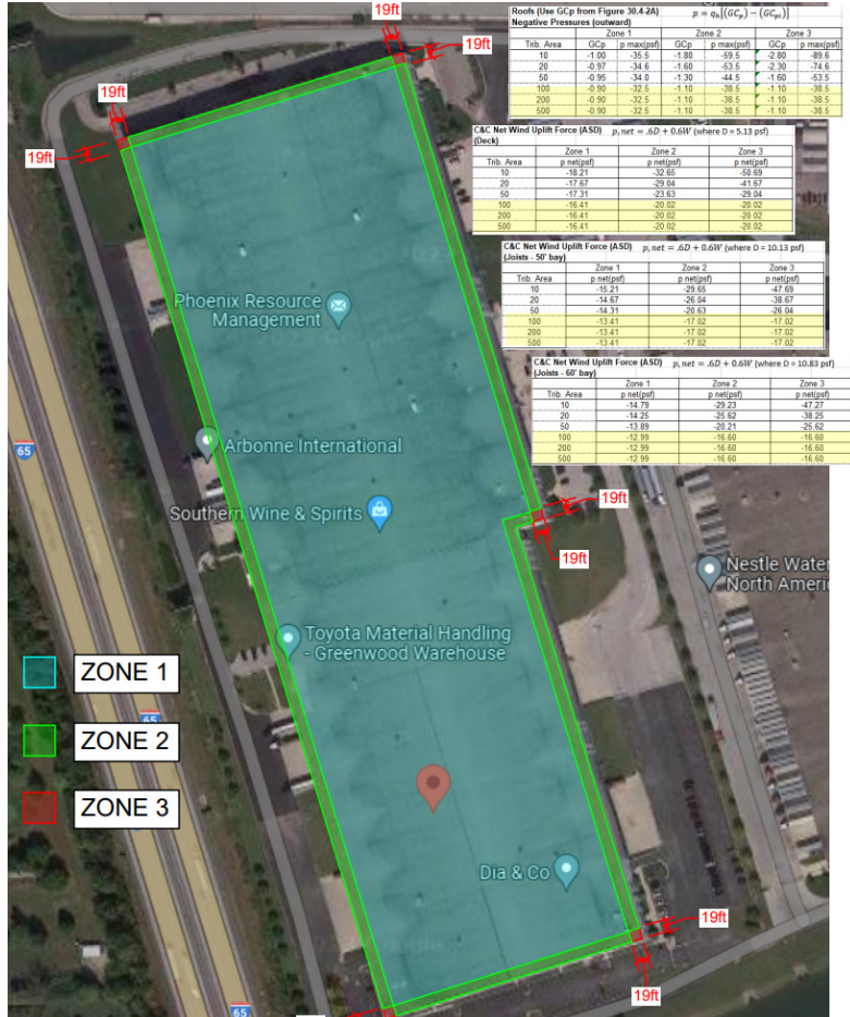
Prologis Solar Panel Study, Indianapolis, Indiana
