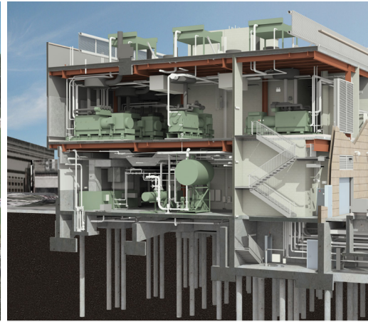
Wishard Hospital Central Utility Plant, Indianapolis, Indiana
